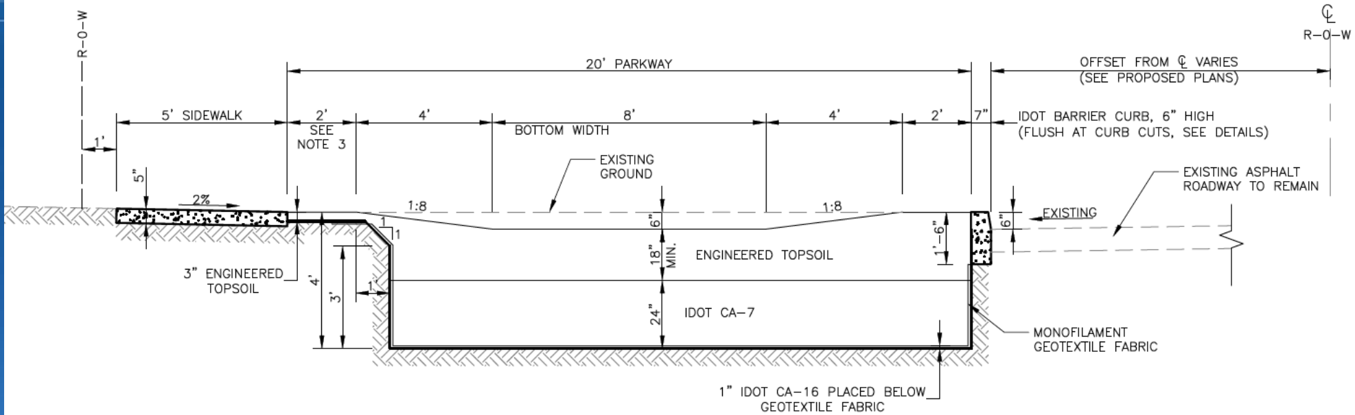
PROPOSED RAIN GARDEN TYPE A TYPICAL SECTION N.T.S.
