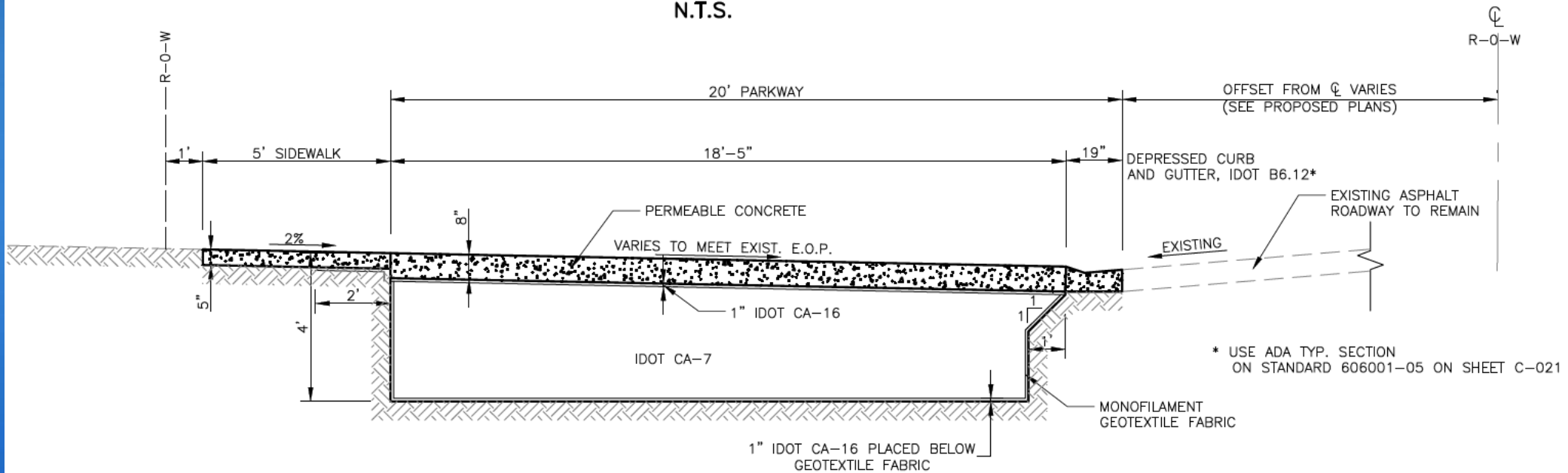
PROPOSED PERMEABLE PAVEMENT TYPICAL SECTION N.T.S.
